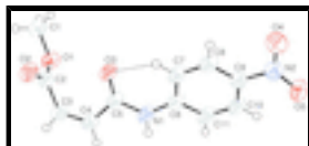
Fig. 1. View of the title compound with the atom numbering scheme. The displacement ellipsoids are drawn at the 50% probability level. H atoms are shown by small circles of arbitrary radii. The dotted line shows intramolecular hydrogen bond.
