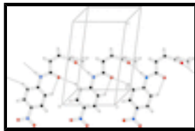
Fig. 2. The partial packing ( PLATON ; Spek, 2009) which shows one dimensional polymeric chain of hydrogen-bonded molecules, extending along the a -axis.
